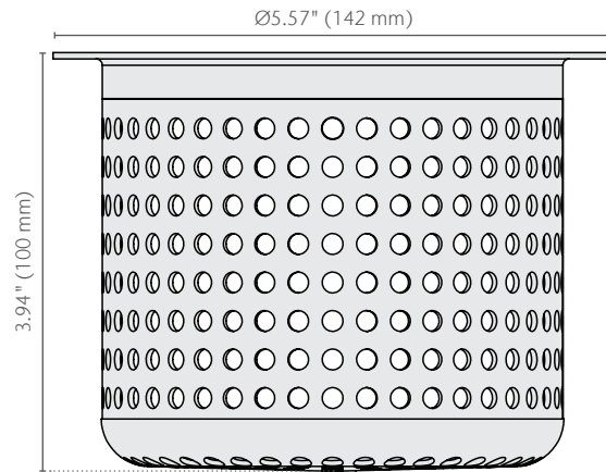
4.0" Debris Strainer Basket
