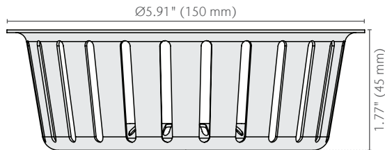
1.8" Debris Strainer Basket
