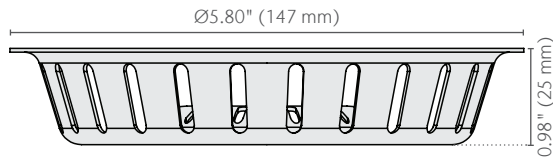
1.0" Debris Strainer Basket
